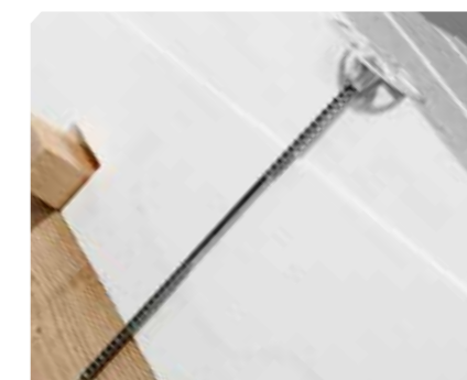
Expansion bolt used to fix the Izodom roof slab.
